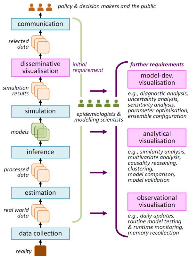
Figure 2: Visualisation tasks can be categorised into four levels according to the complexity of their search spaces. The workflows for epidemiological modelling, especially during an emergency, can benefit significantly from observational, analytical, and model-developmental visualisation in addition to disseminative visualisation. While visualisation can significantly reduce the time required for information acquisition, it can also enable experts to reason with the data in conjunction with their knowledge about, for instance, related facts and events in the reality, shortcomings in data collection and processing, and scientific understanding about the models concerned.
