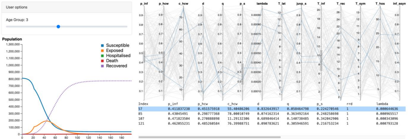
Figure 9: A prototype system for analysing and visualising ensemble data. The parallel coordinate plot (right) allows one to filter input parameters, select a subset of time series to be aggregated, and display the aggregated curves (left).
