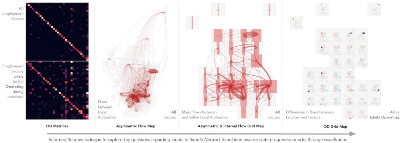
Figure 7: Original origin destination (OD) matrices - travel to work between local authorities in Scotland (top) and those in employment sectors likely to be operating under lockdown (bottom). Asymmetric flow map - all travel to work between local authorities shown in the spatial context, with line widths representing number of daily flows. Flow grid map - all travel to work, shows major flows and has the space to show internal flows. OD grid map - shows differences between travel to work flows in the 'All' and 'Likely Operating' employment sectors. Mini maps show incoming (and internal) flows for each local authority. Blues are negative (lower proportions of workers), reds are positive (higher proportions of commuting). Darker colours show larger differences. Differences are predominantly local at this scale with strong spatial patterns revealed.
