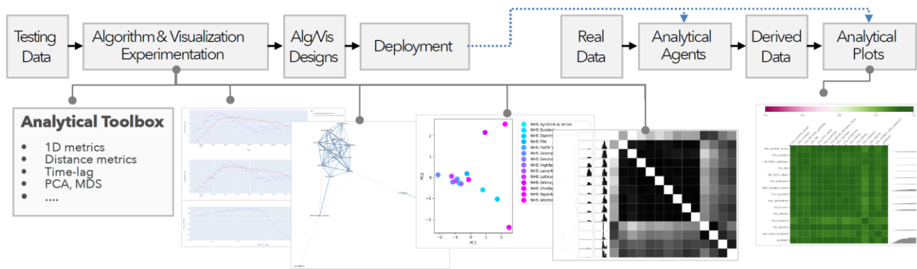
Figure 5: The analytical support team develops and experiments with different analytical algorithms and visual representations (top left) and selects some designs to be deployed on the VIS infrastructure by the generic support team (top right). The lower part of the figure shows examples of analytical visualisations for time series analysis, including time-lag plot, force-directed graph, scatter plot, and heatmap matrix.
