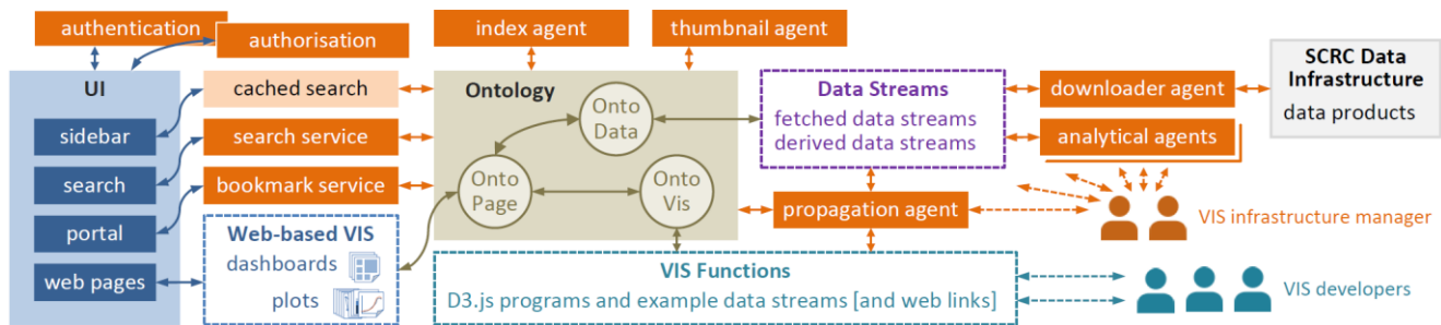
Figure 4: The architecture of the RAMP VIS server, featuring its ontology, agents, and services, and their relationships with the UI, web pages (dashboards and plots), VIS functions (programs and test data), fetched and derived data streams, and SCRC data infrastructure.
