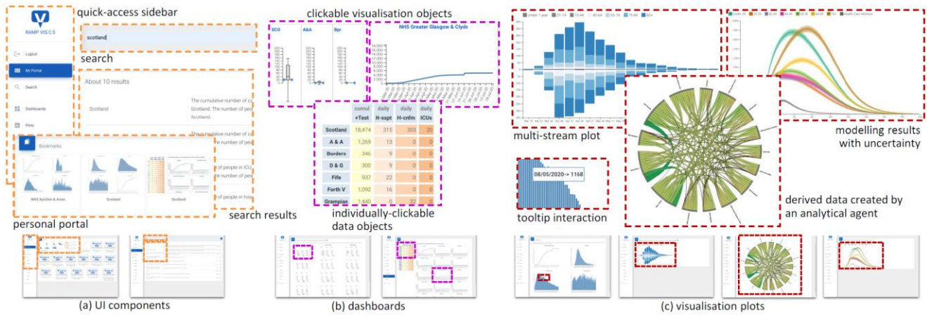
Figure 3: The RAMP VIS server ( vis.scruc.uk ) provides users with a user interface (with search facility, personal portal, etc.), a collection of dashboards (with clickable visual and data objects), and various plots for visualising the data hosted by the SCRC data infrastructure.
